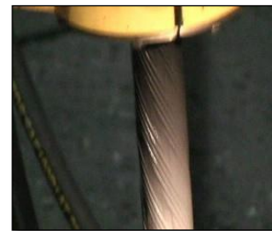
Dynagard LVL Being Applied to a Mine's Slope Rope. Model JU16L, Highland Mining, Kentucky USA
